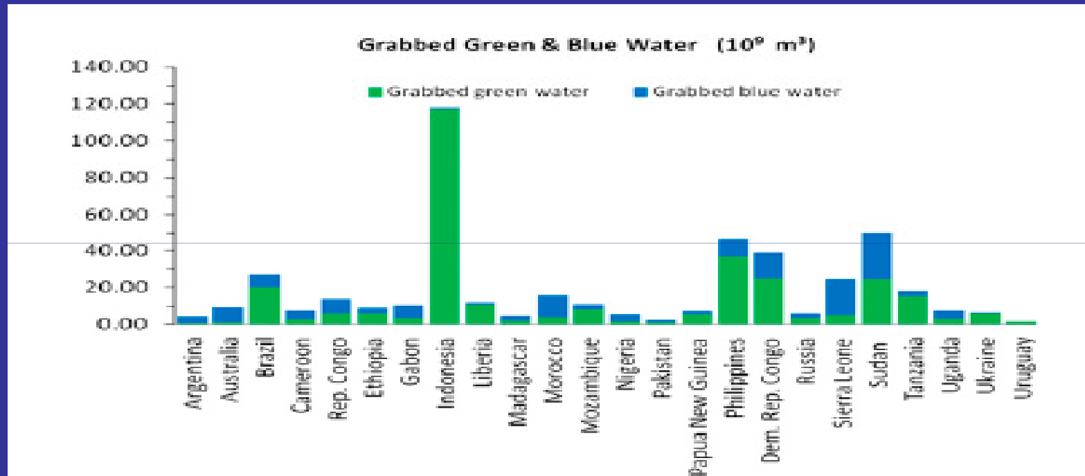
Fig. 3. Water grabbing in the 24 most land-grabbed countries (Table 1). Green and maximum blue water grabbing (Table 3).
